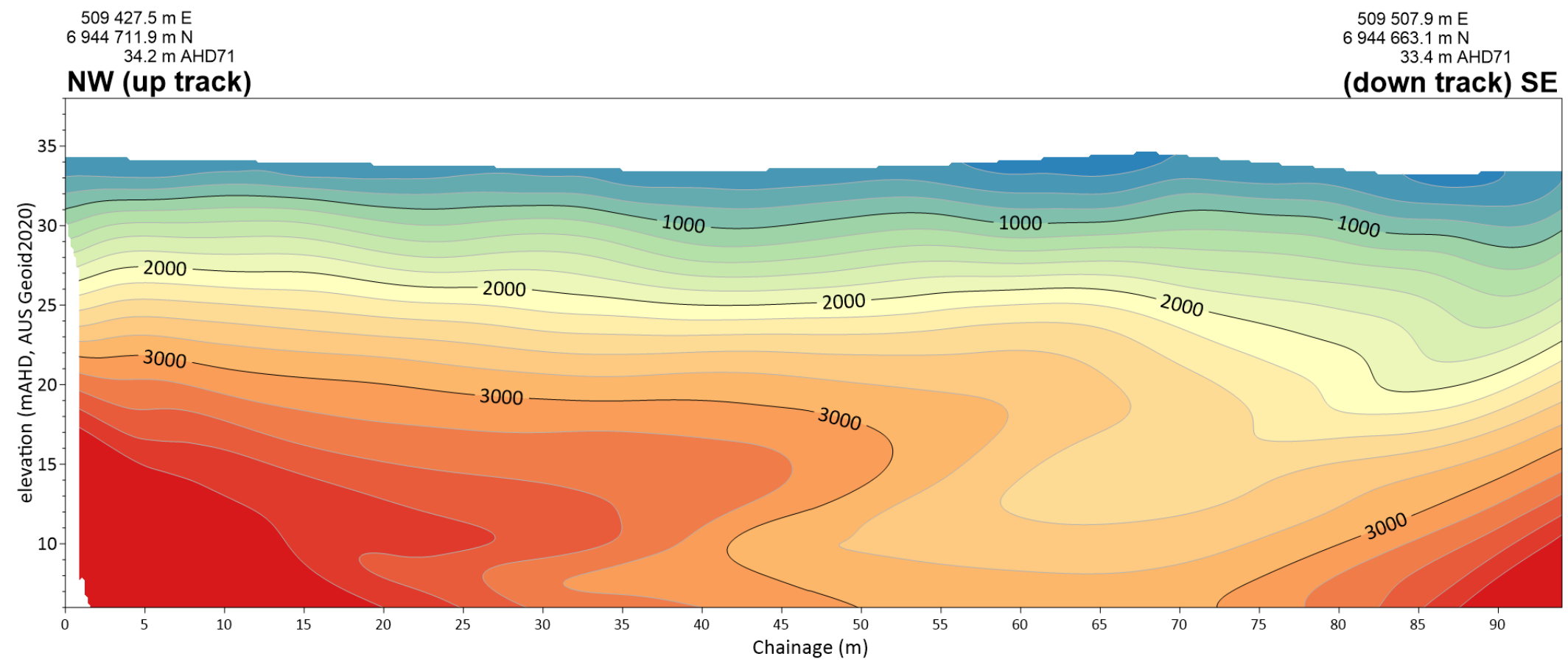
Seismic Line SR AU-GP 111
